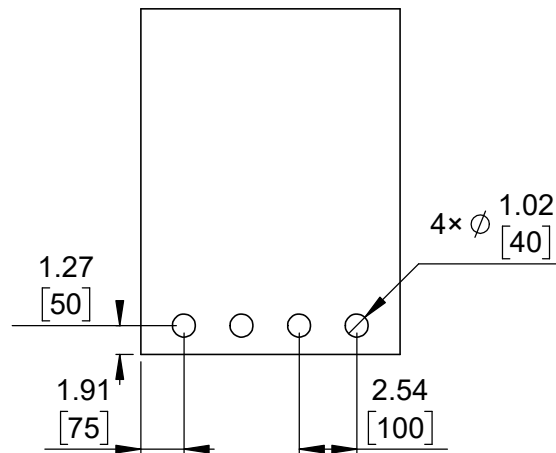
2 Connector callouts (bottom view) Scale 3:1
